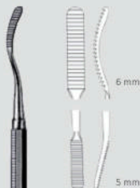
INS-23-0591-02 18.5 cm / 7 1/4" Double ended, plain serrations
